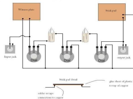
Fig 1 Radionics Schema 2.1.2.2. History of Radionics
