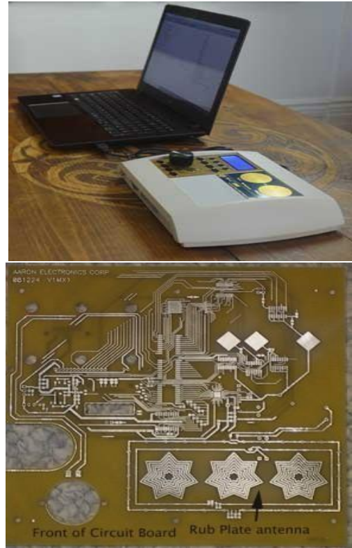
Fig 2 Radionics Machine SE5-1000
